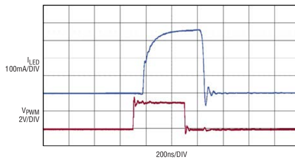
INFINITE PERSISTENCE V IN = 12V f PWM = 100Hz
